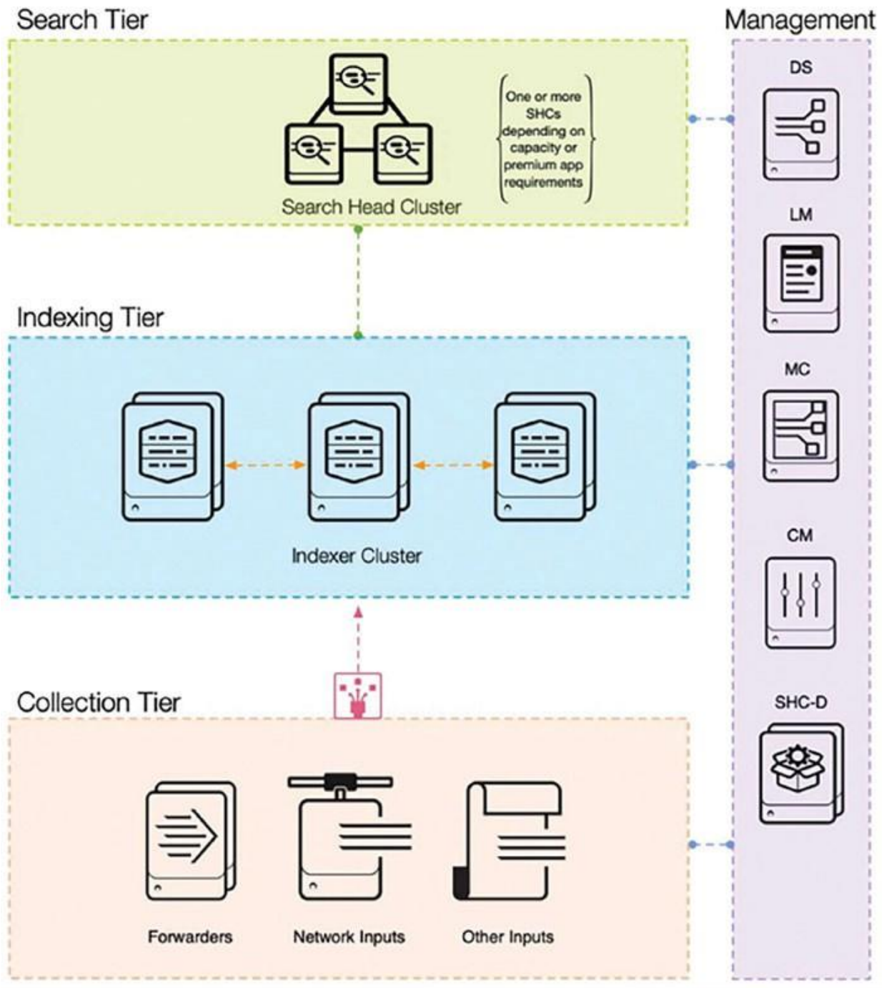
Figure 4.2: Data ingestion in Splunk (Source: Get Answers from Your Data with Cisco UCS Integrated Infrastructure for Splunk Enterprise. (2023, March 20). Cisco.
