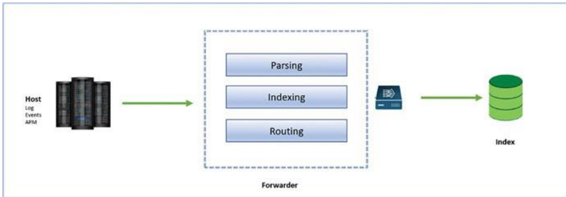
Figure 2.2: Splunk Forwarder
