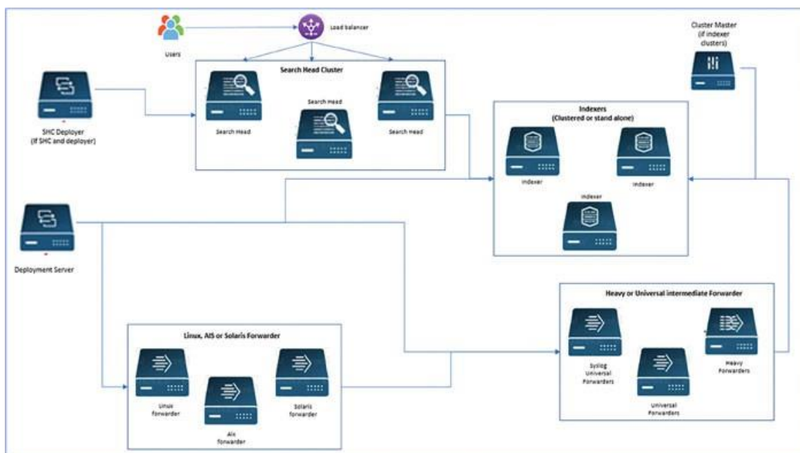
Figure 2.3: Splunk Architecture
