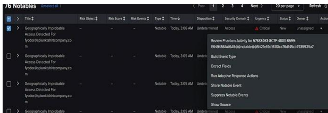
Figure 6.6: Notable events
