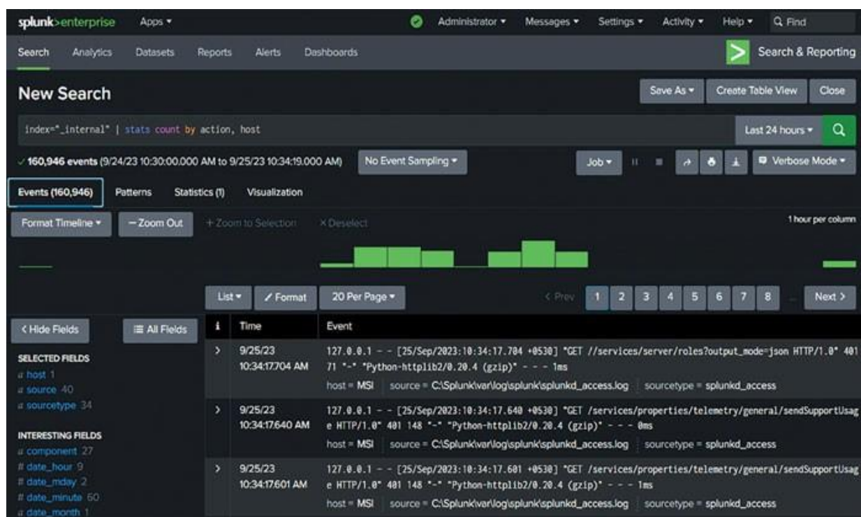
Figure 1.2: Splunk Search
